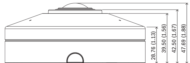
Afmetingen in mm (inch)
